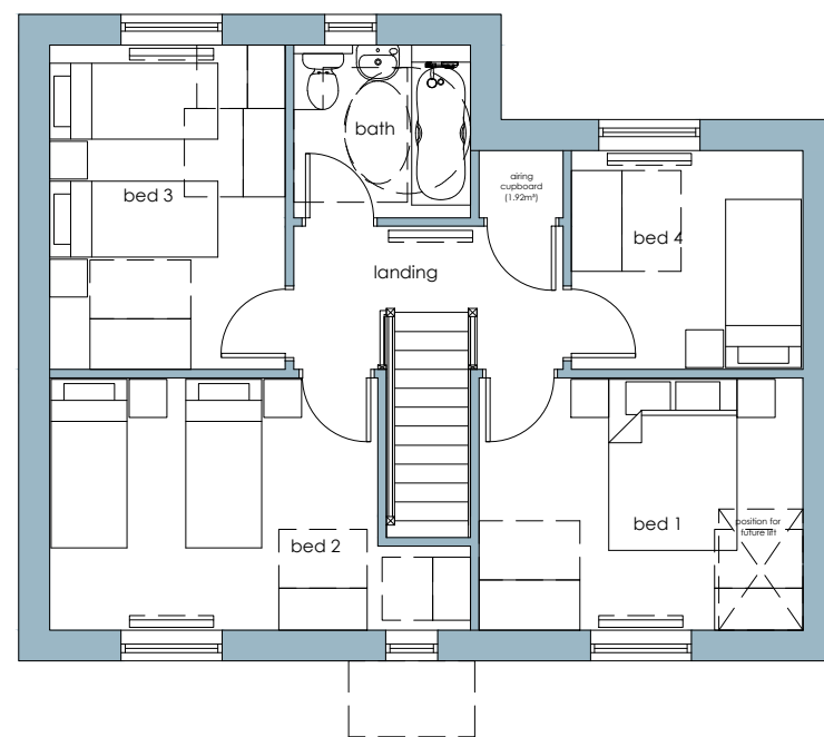
FIRST FLOOR PLAN Typical 4 Bed House Type
