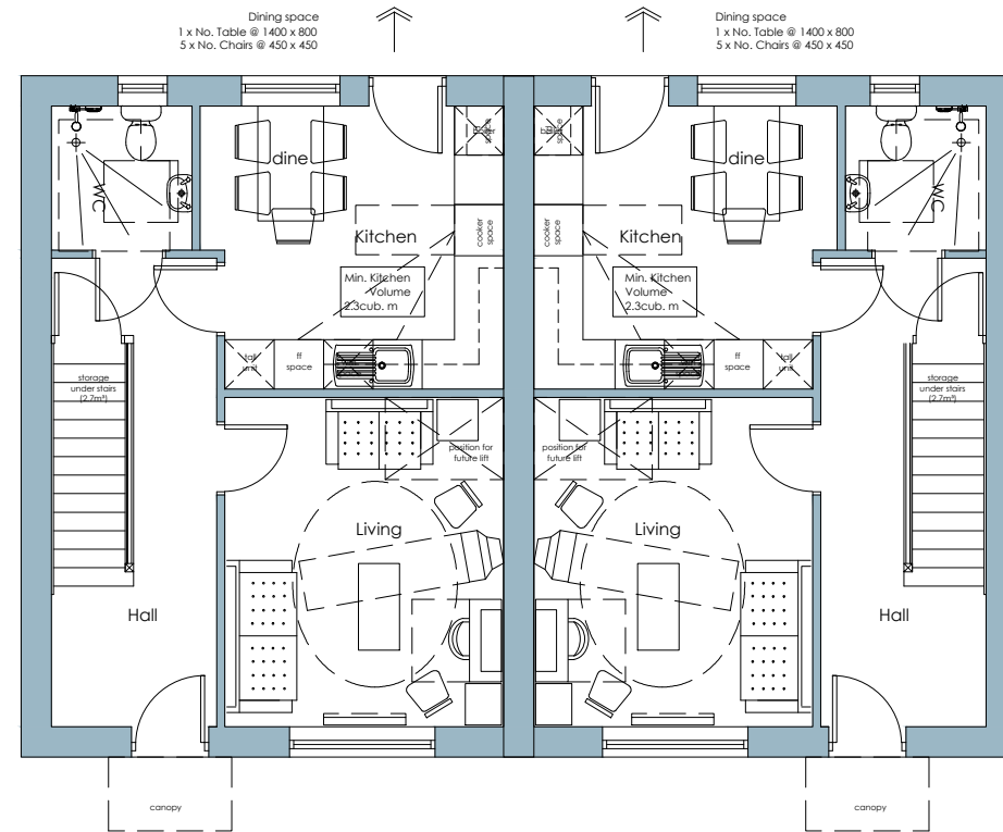
GROUND FLOOR PLAN Typical 2 Bed House
